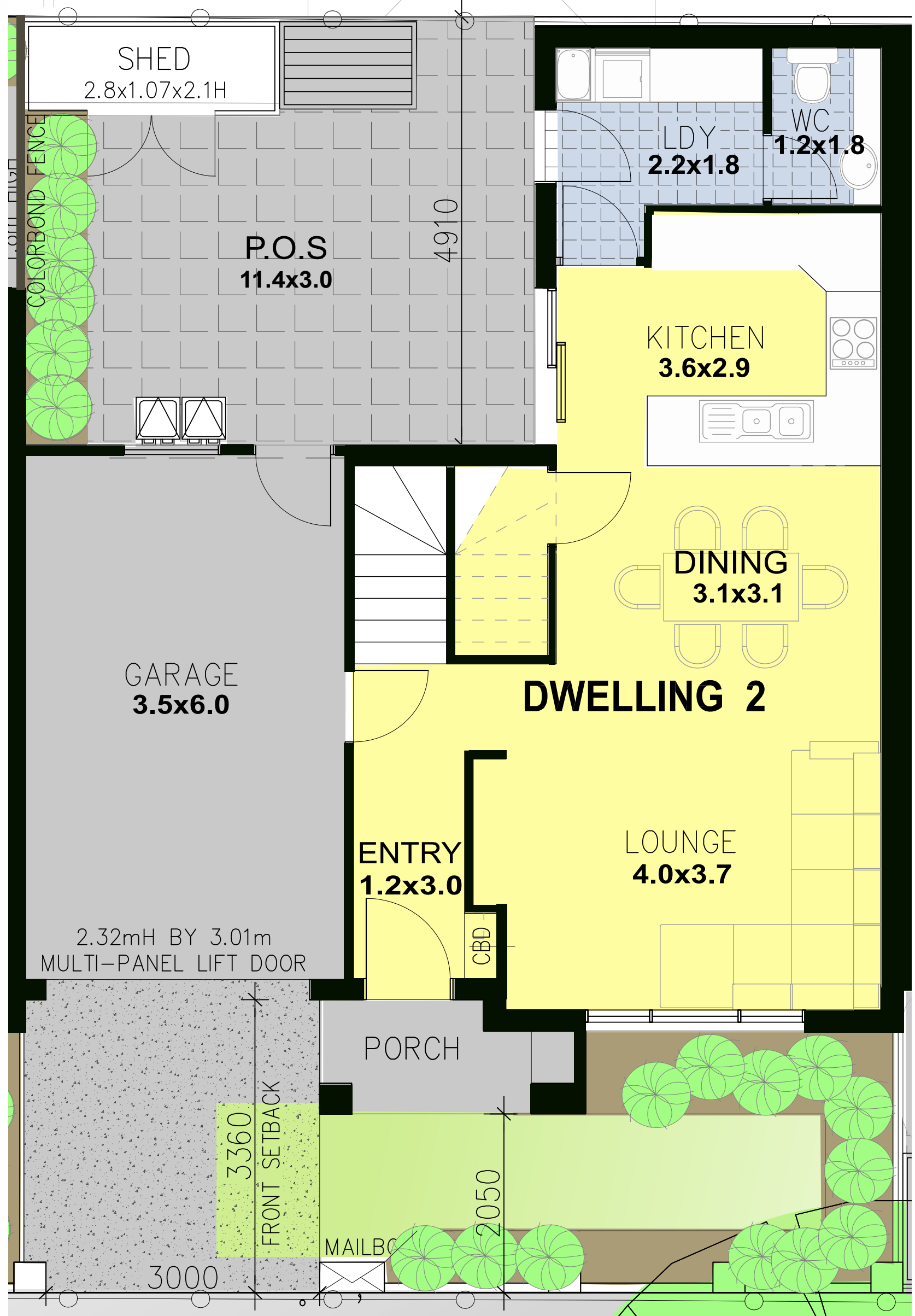
1ST FLOOR
